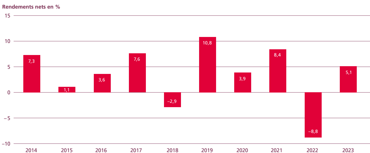
Illustration C-1: Rendements nets 2014–2023
